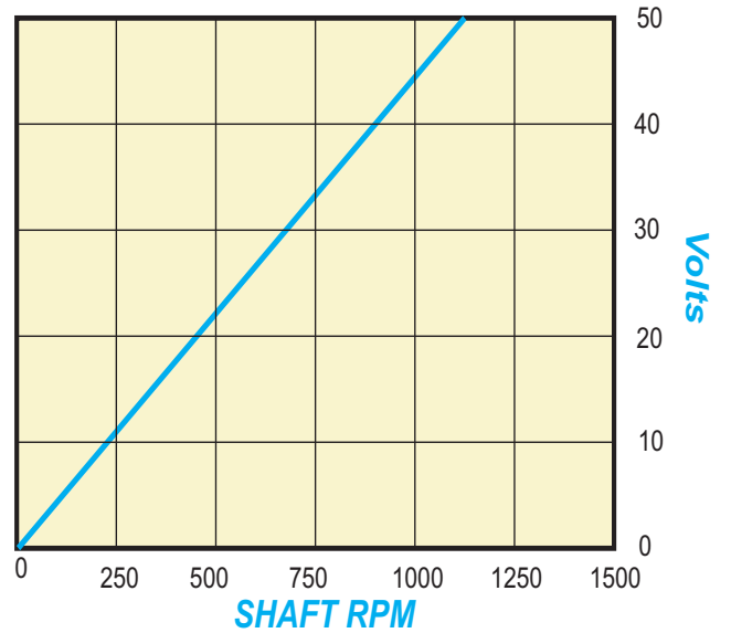
OPEN CIRCUIT VOLTAGE CURVE
