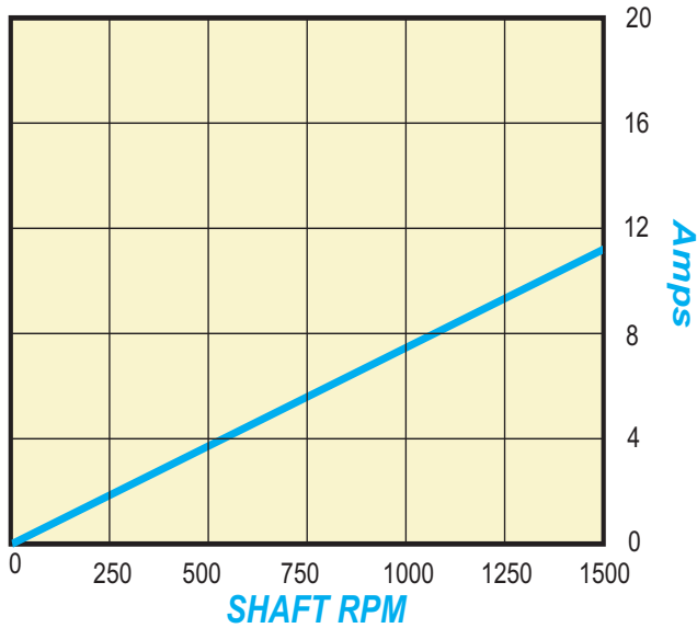
SHORT CIRCUIT AMPERAGE CURVE
